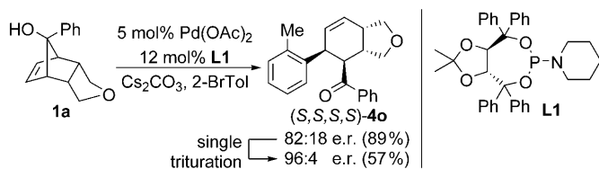
Scheme 6. Initial result for an enantioselective version of arylation ring-opening.
