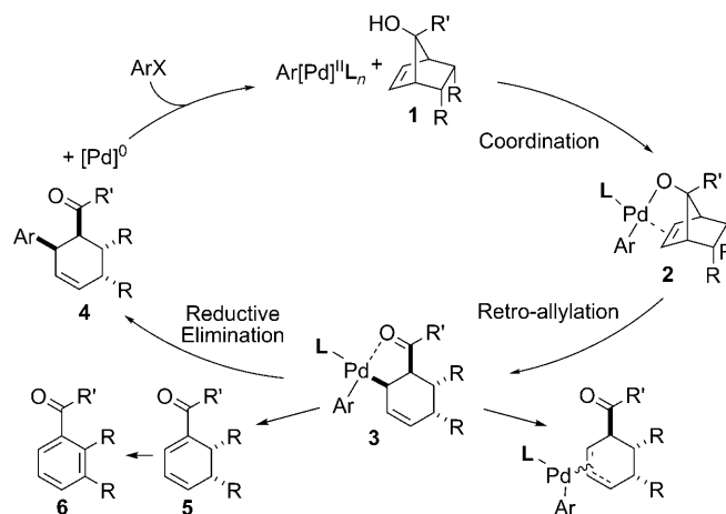
Scheme 1. Palladium-catalyzed arylative ring-opening of norbornenols.
