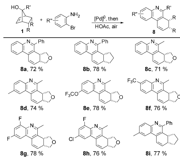
Scheme 4. Scope for quinolines 8 . Reaction conditions: 1 (0.05 mmol), ArBr (2 equiv), Cs 2 CO 3 (1.5 equiv), Pd(OAc) 2 (5 mol %), S-Phos (12 mol %); 0.15 M in toluene, 100 °C, 12 h, then AcOH (15 equiv), 23 °C, 2 h.
