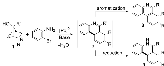
Scheme 3. Domino cyclization of norbornenols 1 with o -bromoanilines.
