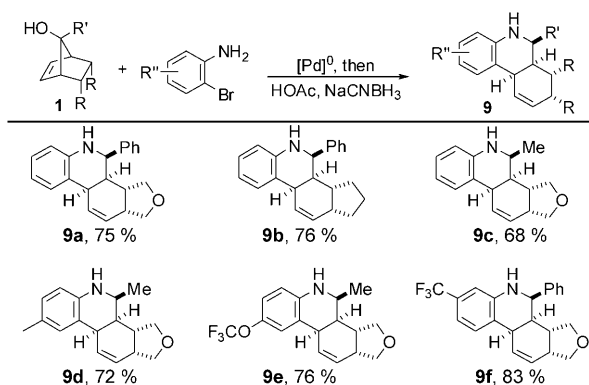
Scheme 5. Scope for tetrahydroquinolines 9 . Reaction conditions: 1 (0.05 mmol), ArBr (2 equiv), Cs 2 CO 3 (1.5 equiv), Pd(OAc) 2 (5 mol %), S-Phos (12 mol %); 0.15 M in dioxane, 100 °C, 3 h, then NaCNBH 3 (3 equiv), AcOH (5 equiv), 23 °C, 2 h.
