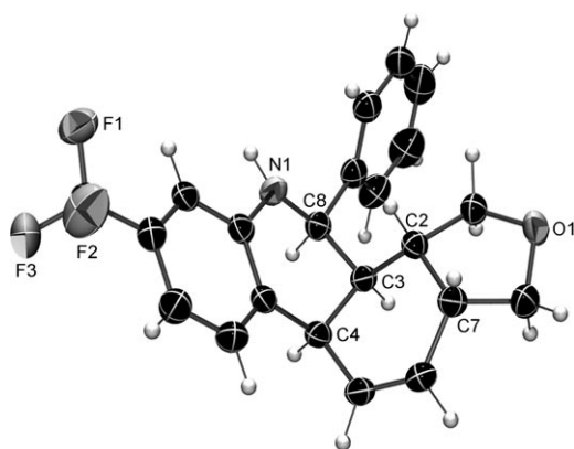
Figure 1. ORTEP representation of 9f . The thermal ellipsoids are drawn at a 50% probability.
